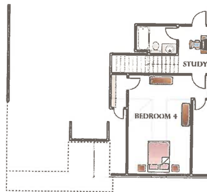
2 nd Floor
